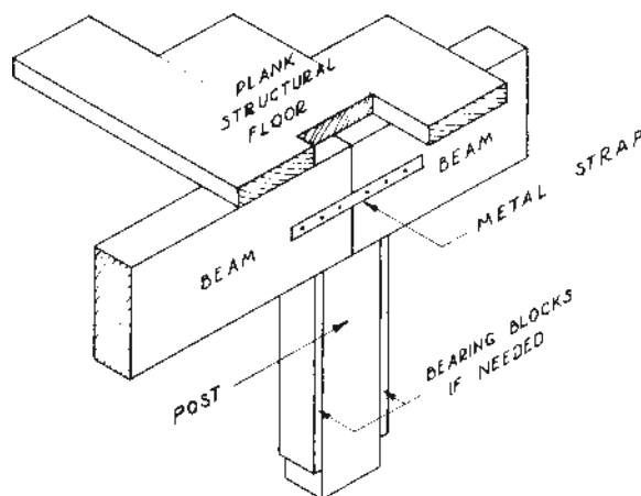
Figure 11 Solid Beam Bearing Over Basement Post
